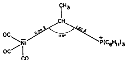
Fig. 3. X-ray molecular structure of a nickel carbonyl ylide complex.
