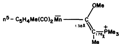
Fig. 6. X-ray molecular structure of ^5\eta -cyclopentadienylmanganese carbonyl ylide acyl complex.
