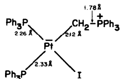
Fig. 7. X-ray molecular structure of iodobis(triphenylphosphine)methylenetriphenylphosphoraneplatinum(II).
