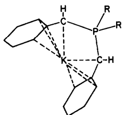
Fig. 2. X-ray structure of a potassium benzyliide.
